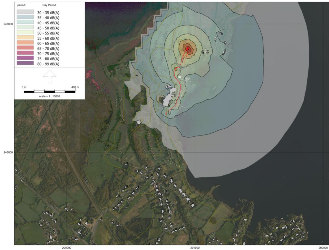
Figure A11-I-20 Construction phase L_{Aeq} 1 h contours at 2 m height – Construction scenario 20.
