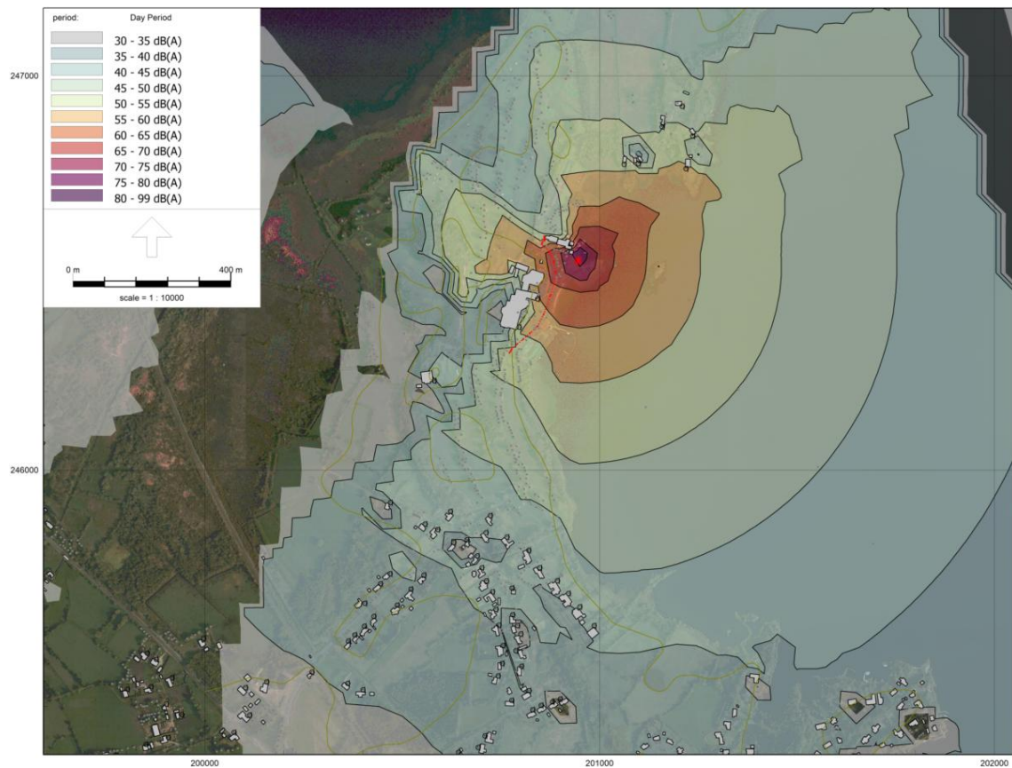
Figure A11-I-1 Construction phase L_{Aeq\ 1\ h} contours at 2 m height – Construction scenario 1.
