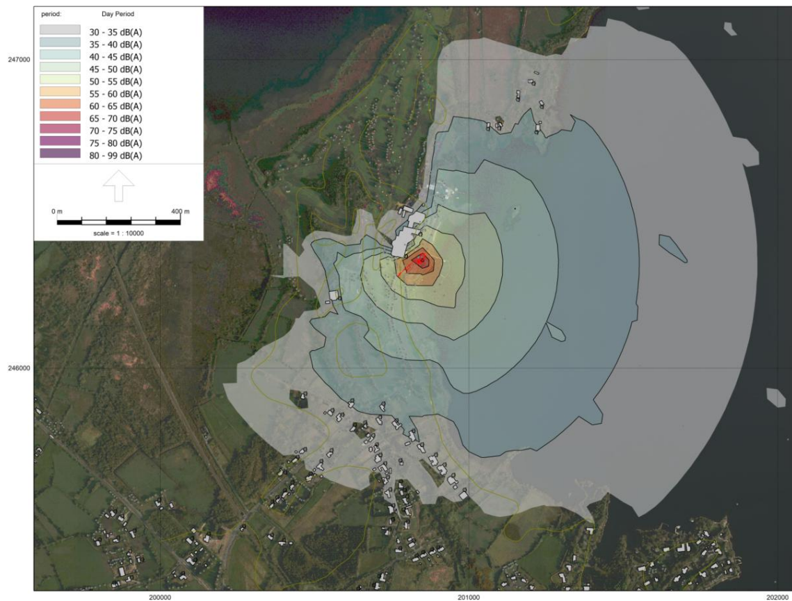
Figure A11-I-15 Construction phase L_{Aeq\ 1\ h} contours at 2 m height – Construction scenario 15.
