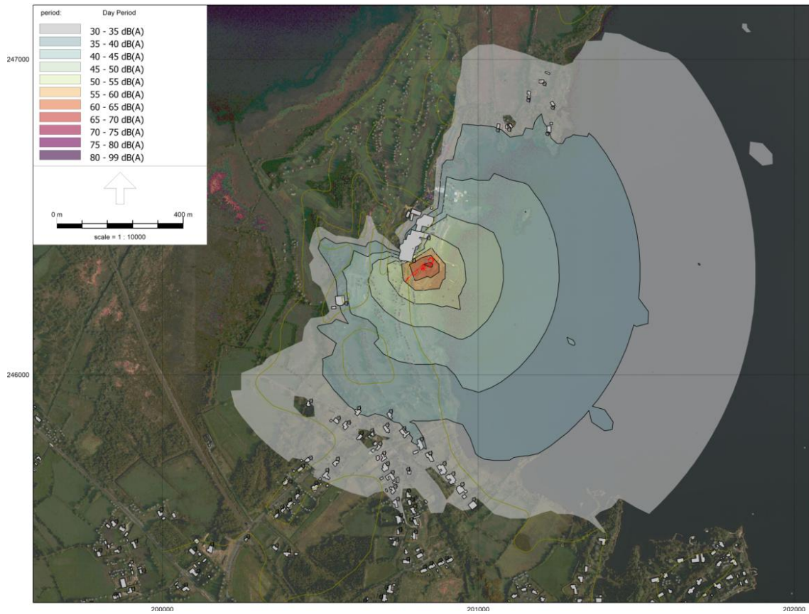
Figure A11-I-16 Construction phase L_{Aeq\ 1\ h} contours at 2 m height – Construction scenario 16.
