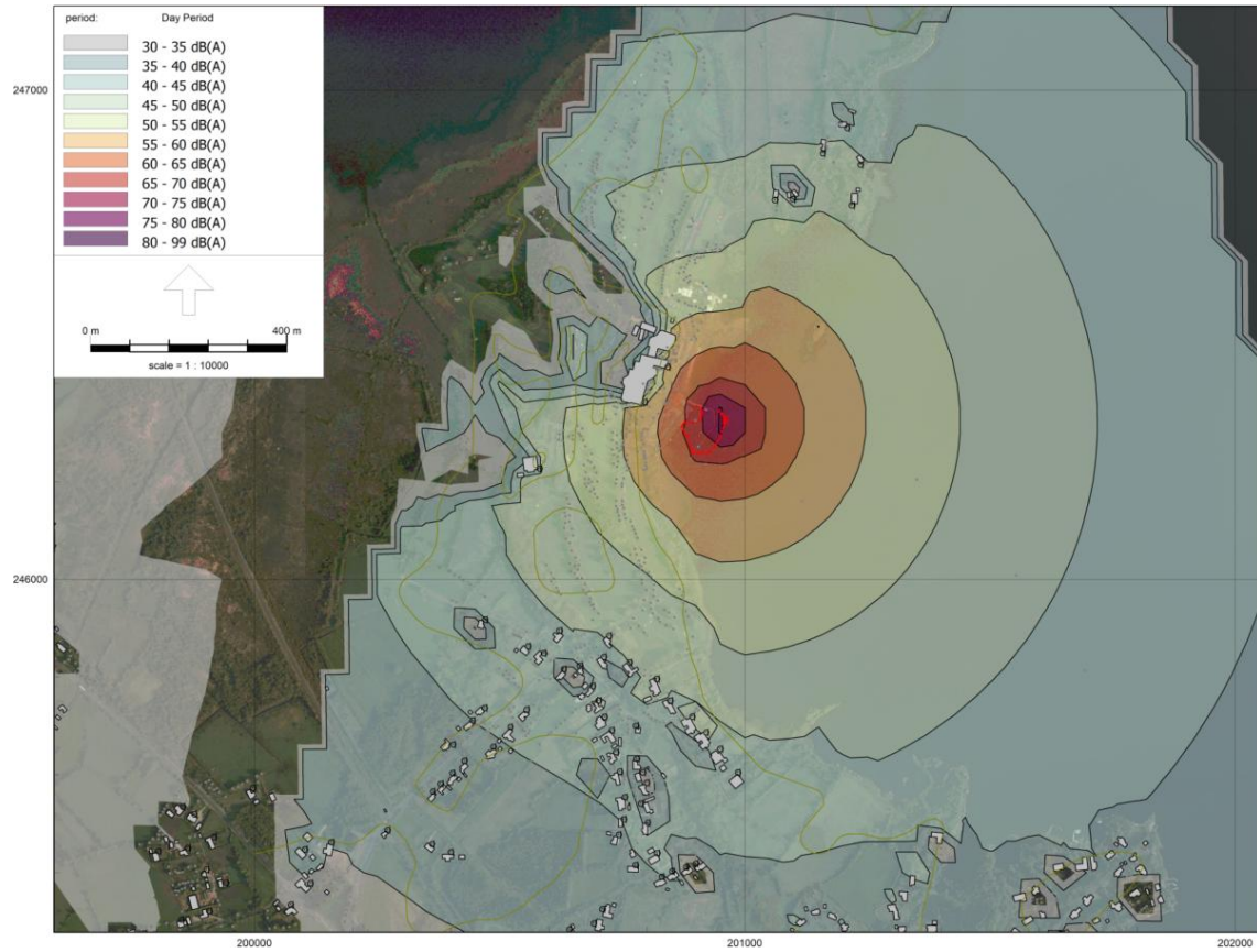
Figure A11-I-10 Construction phase L_{Aeq\ 1\ h} contours at 2 m height – Construction scenario 10.
