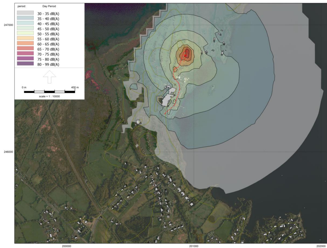
Figure A11-1-22 Construction phase L_{Aeq} 1 h contours at 2 m height – Construction scenario 22.
