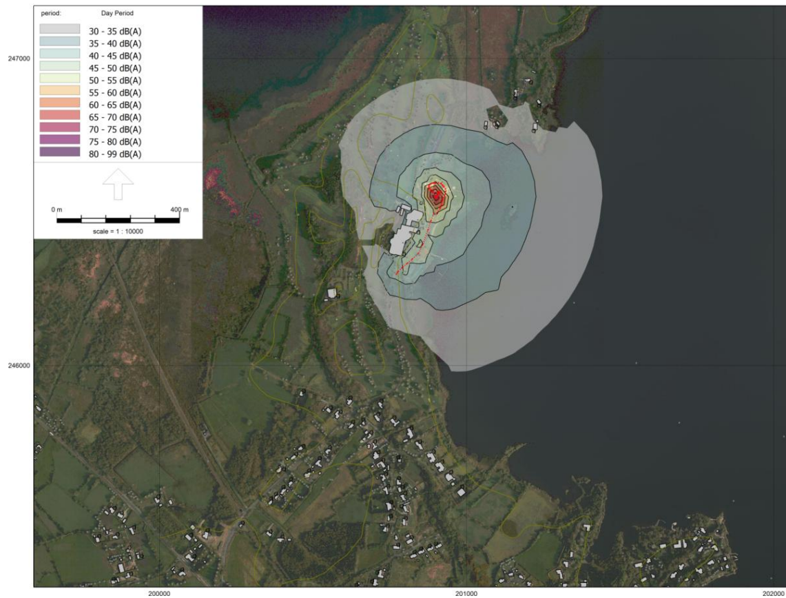
Figure A11-1-7 Construction phase L_{Aeq\ 1\ h} contours at 2 m height – Construction scenario 7.
