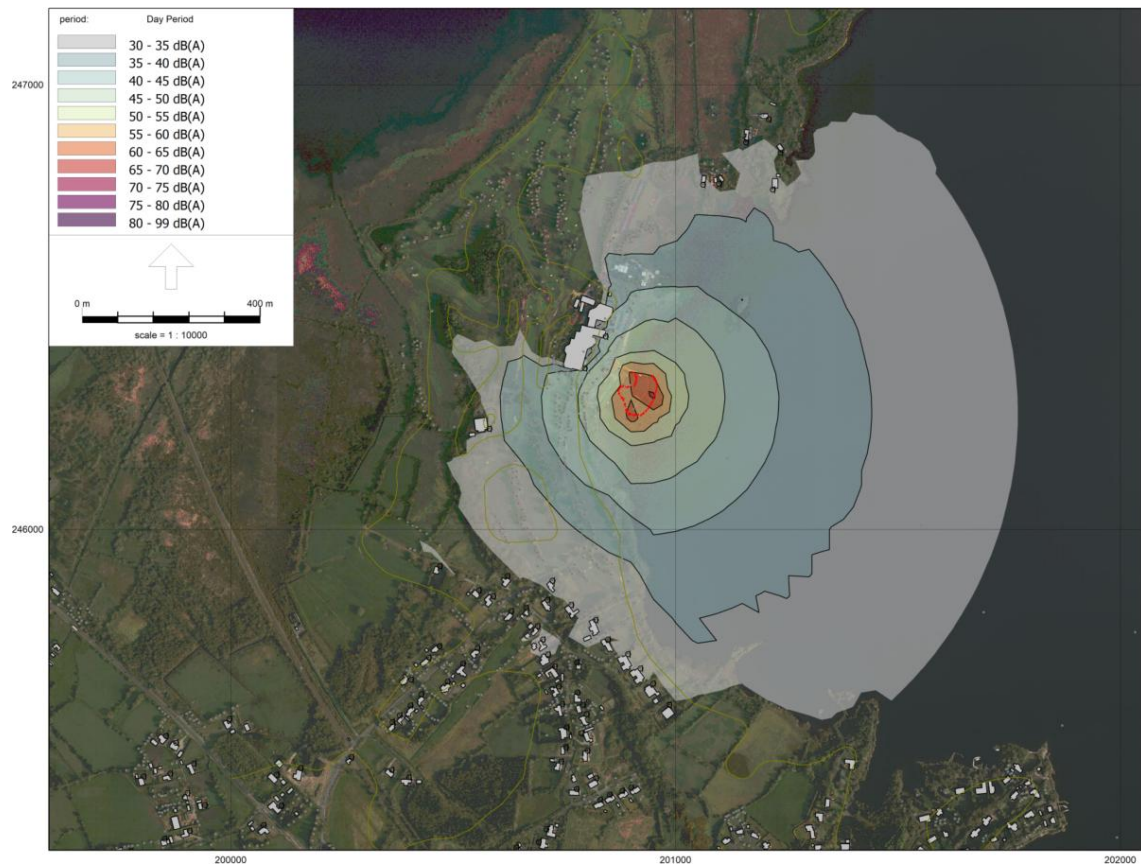
Figure A11-I-9 Construction phase L_{Aeq\ 1\ h} contours at 2 m height – Construction scenario 9.
