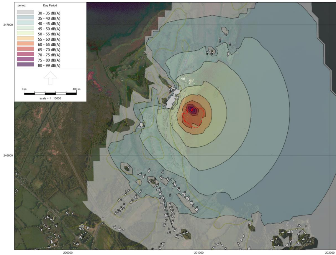
Figure A11-I-11 Construction phase L_{Aeq\ 1\ h} contours at 2 m height – Construction scenario 11.
