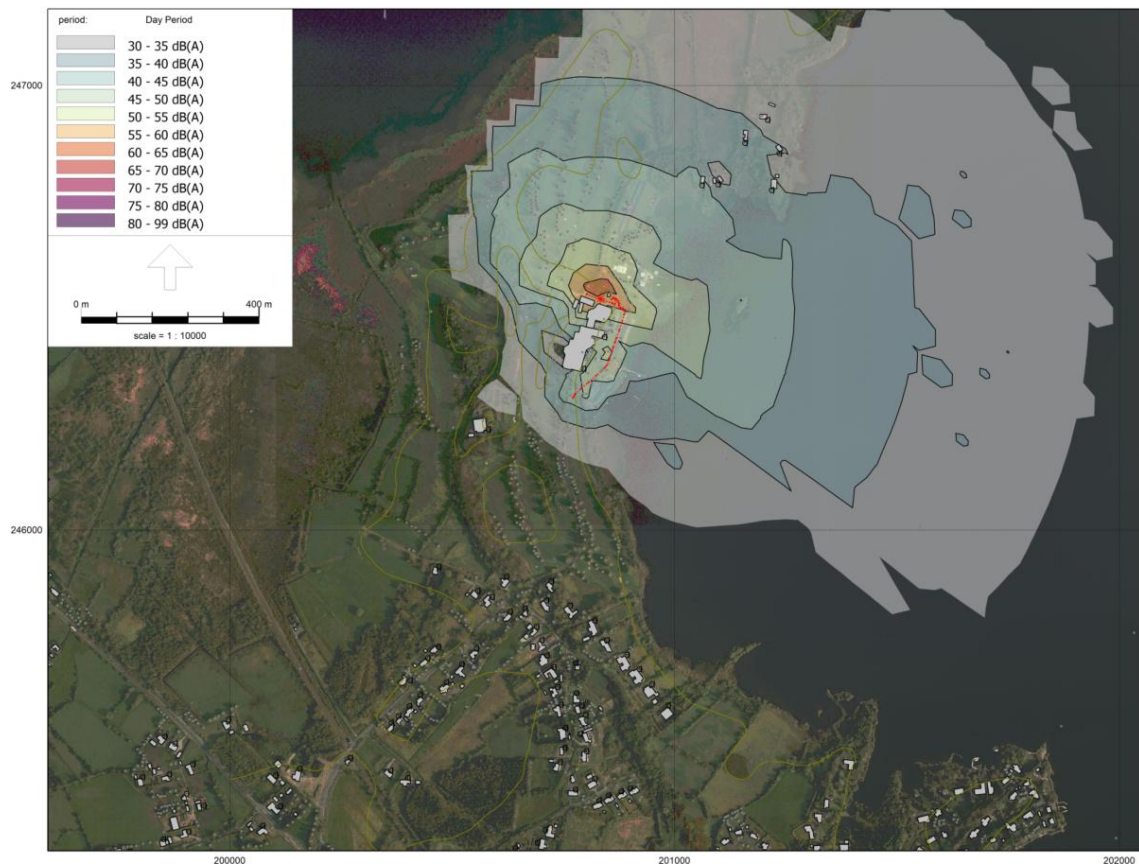
Figure A11-I-18 Construction phase L_{Aeq\ 1\ h} contours at 2 m height – Construction scenario 18.
