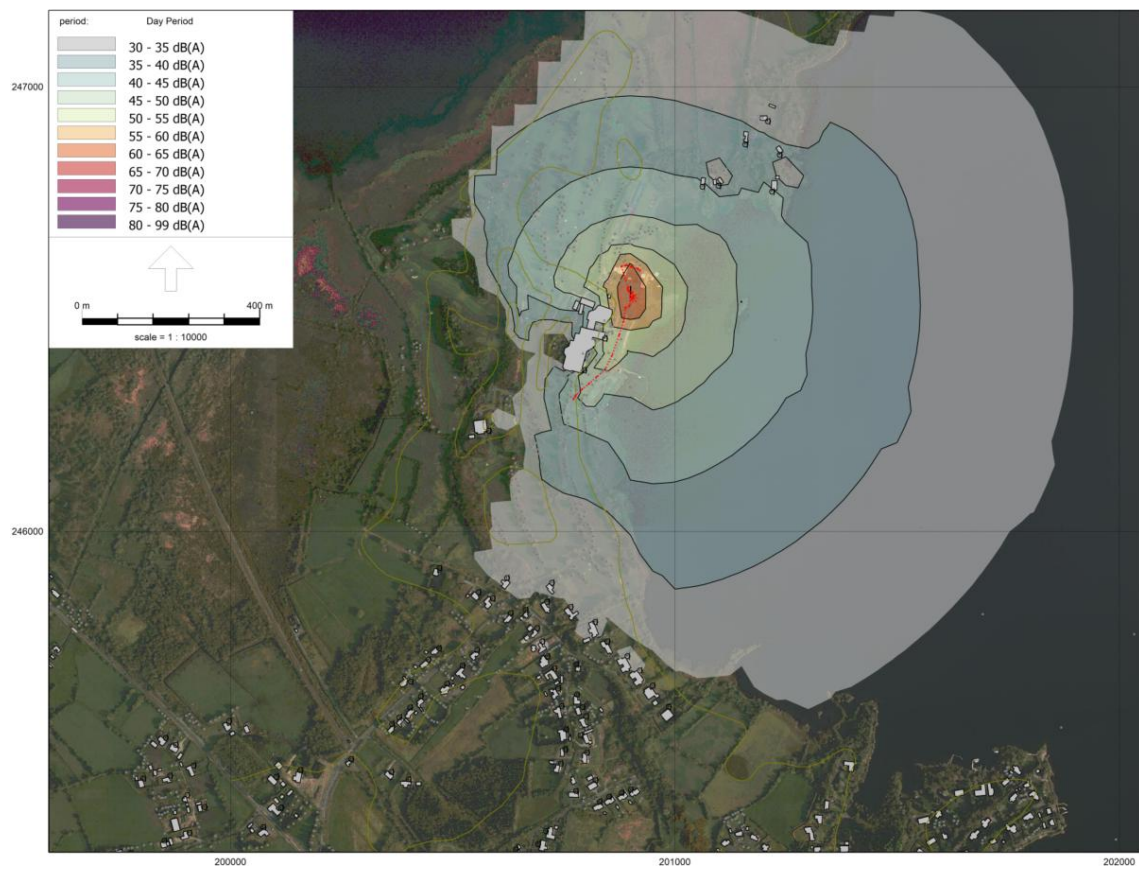
Figure A11-I-4 Construction phase L_{Aeq\ 1\ h} contours at 2 m height – Construction scenario 4.
