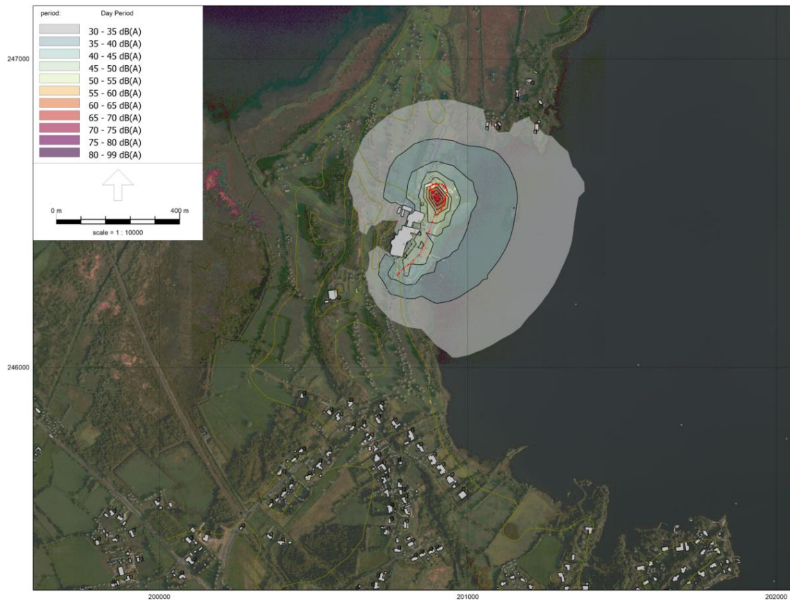
Figure A11-I-6 Construction phase L_{Aeq\ 1\ h} contours at 2 m height – Construction scenario 6.
