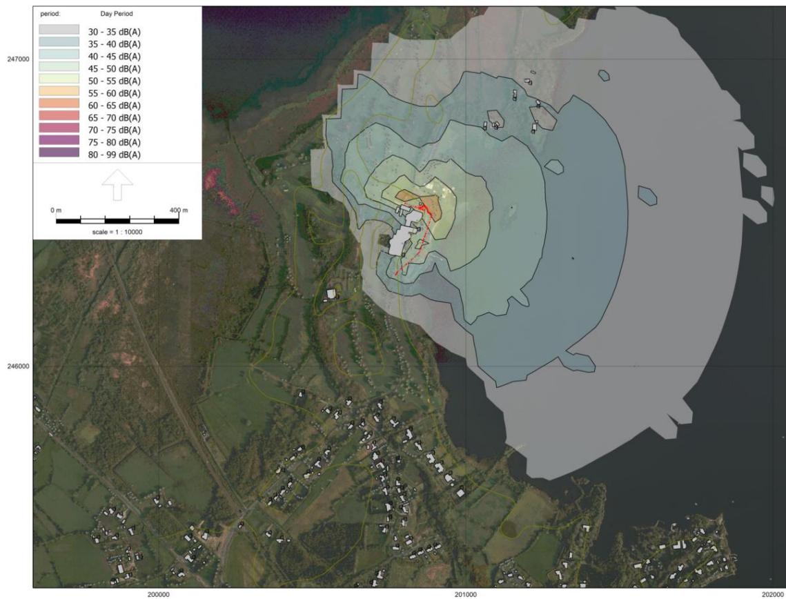
Figure A11-I-19 Construction phase L_{Aeq} 1 h contours at 2 m height – Construction scenario 19.
