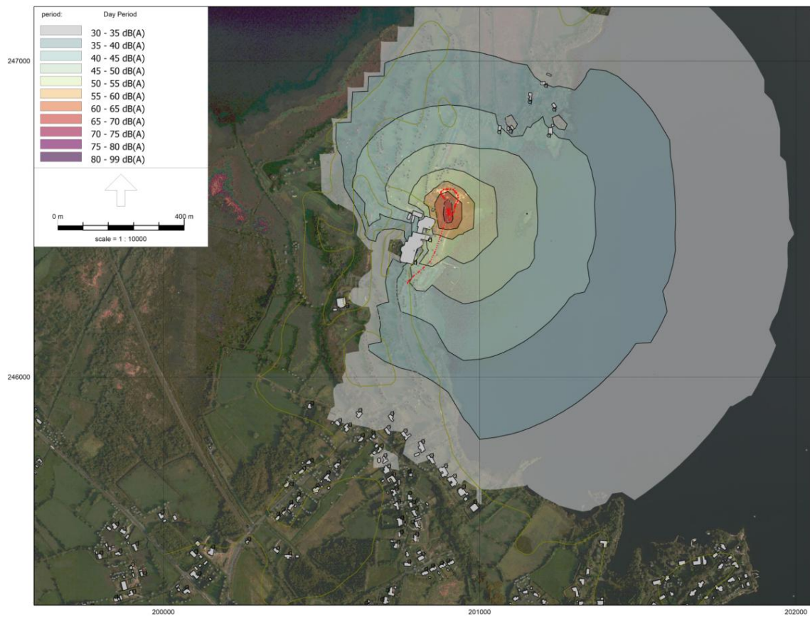
Figure A11-I-5 Construction phase L_{Aeq\ 1\ h} contours at 2 m height – Construction scenario 5.
