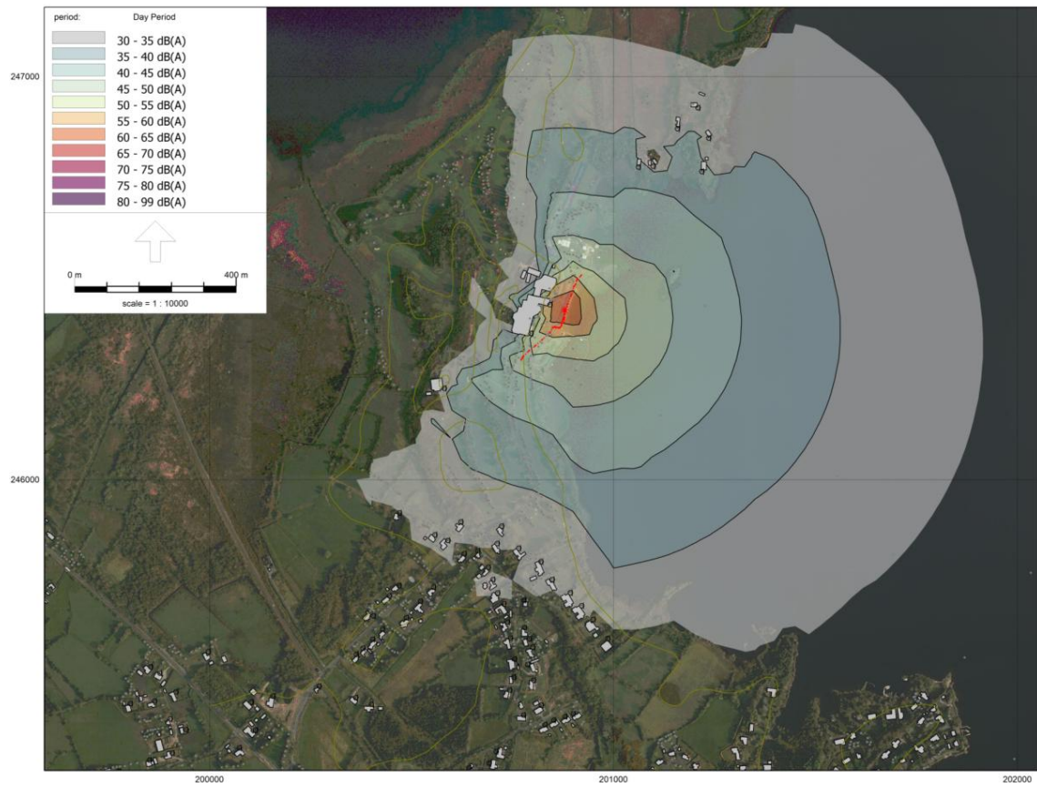
Figure A11-I-12 Construction phase L_{Aeq\ 1\ h} contours at 2 m height – Construction scenario 12.
