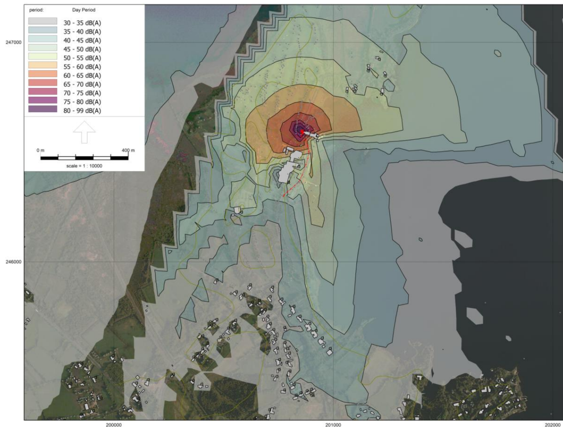
Figure A11-I-3 Construction phase L_{Aeq\ 1\ h} contours at 2 m height – Construction scenario 3.
