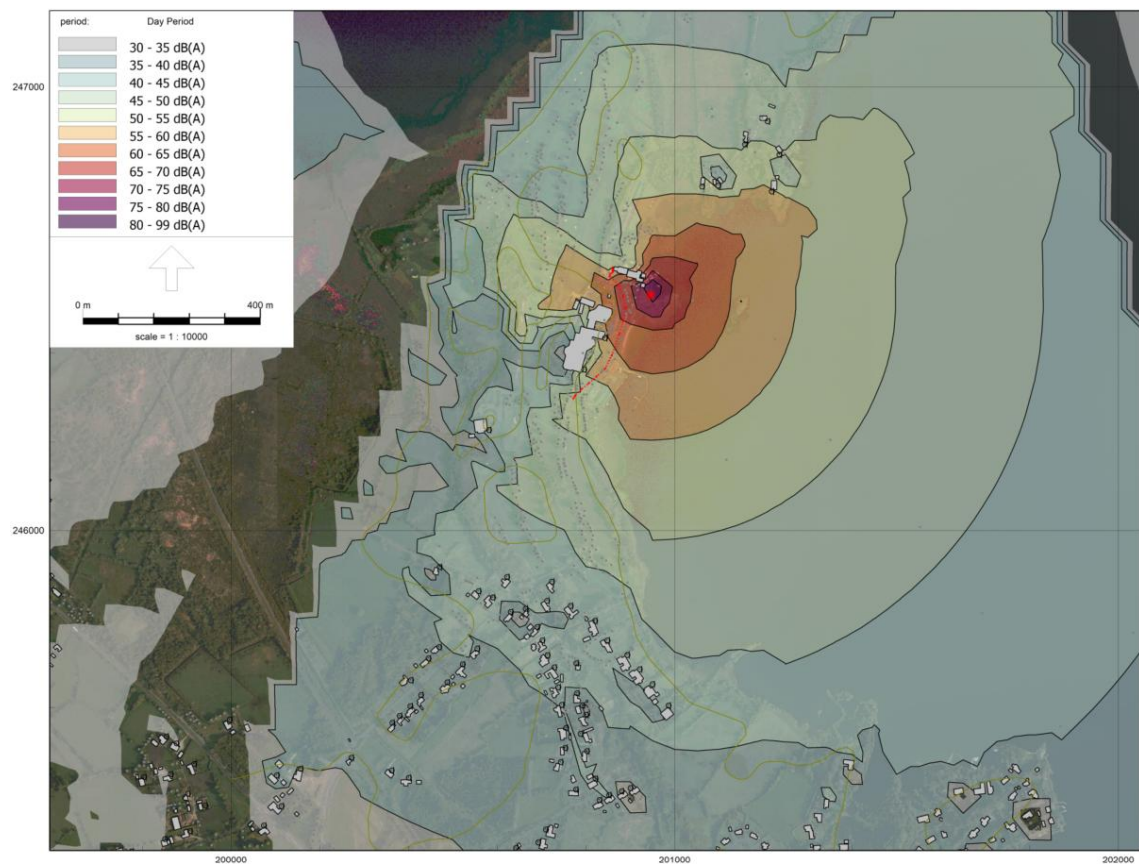
Figure A11-I-2 Construction phase L_{Aeq\ 1\ h} contours at 2 m height – Construction scenario 2.
