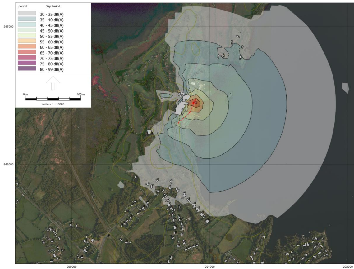
Figure A11-I-13 Construction phase L_{Aeq\ 1\ h} contours at 2 m height – Construction scenario 13.
