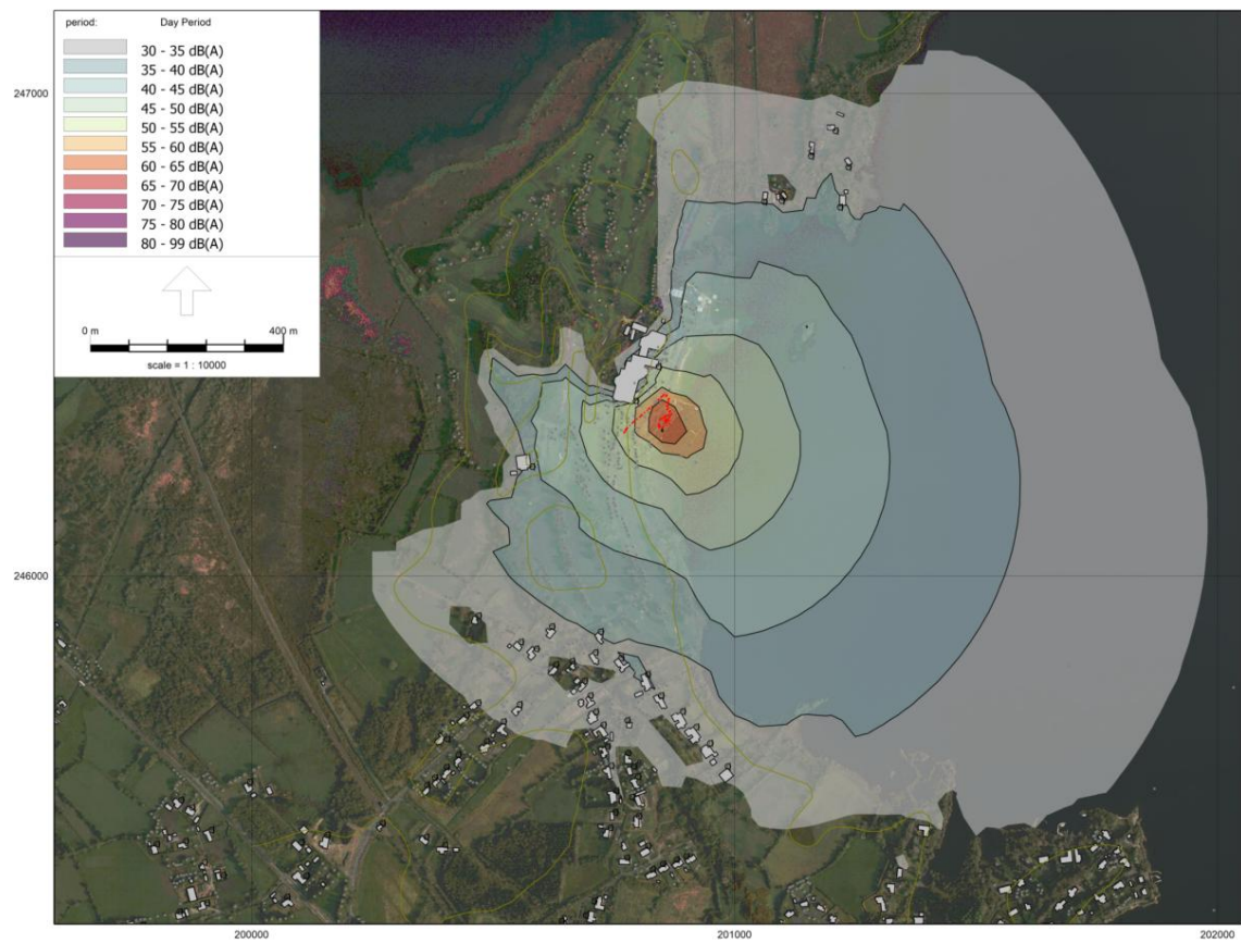
Figure A11-1-8 Construction phase L_{Aeq\ 1\ h} contours at 2 m height – Construction scenario 8.
