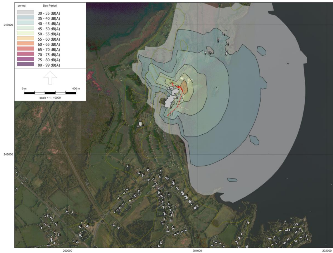
Figure A11-I-17 Construction phase L_{Aeq\ 1\ h} contours at 2 m height – Construction scenario 17.
