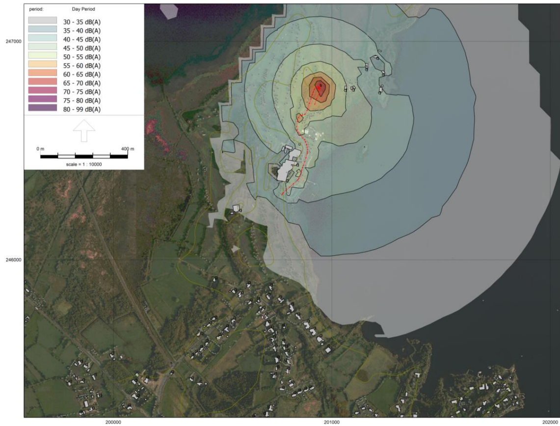
Figure A11-1-21 Construction phase L_{Aeq} 1 h contours at 2 m height – Construction scenario 21.
