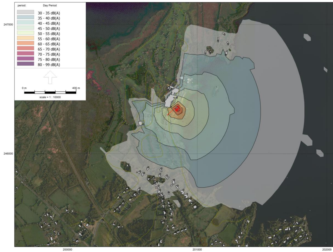
Figure A11-I-14 Construction phase L_{Aeq\ 1\ h} contours at 2 m height – Construction scenario 14.
